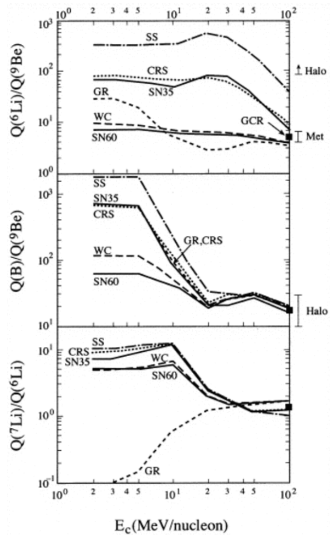
Fig. 10. from Isotopic Lithium Abundances in Nine Halo Stars Smith, Lambert, & Nissen 1998 ApJ 506 405 doi:10.1086/306238 https://dx.doi.org/10.1086/306238 © 1998. The American Astronomical Society. All rights reserved. Printed in U.S.A.
