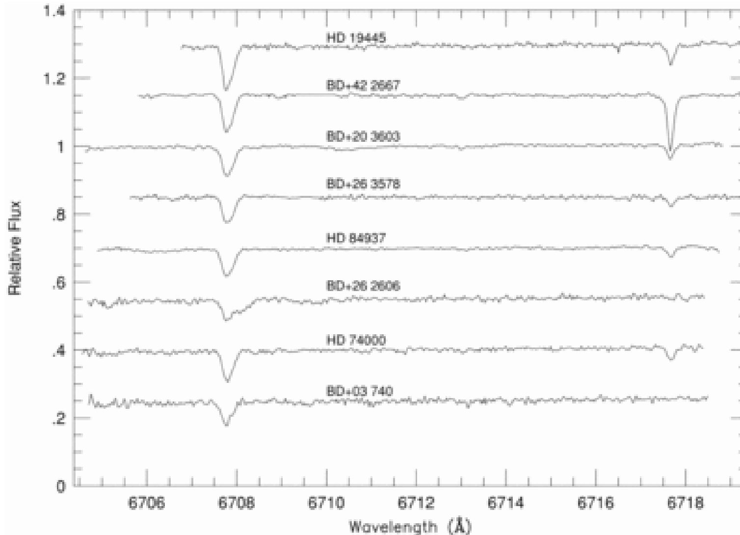
Fig. 1. from Isotopic Lithium Abundances in Nine Halo Stars Smith, Lambert, & Nissen 1998 ApJ 506 405 doi:10.1086/306238 https://dx.doi.org/10.1086/306238 © 1998. The American Astronomical Society. All rights reserved. Printed in U.S.A.
