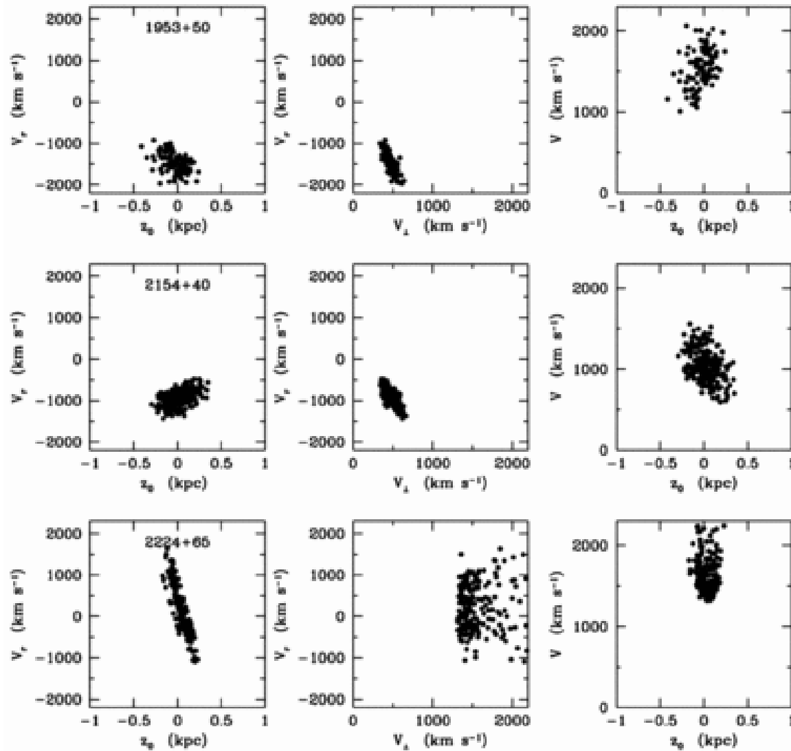
Fig. 9. from Neutron Star Population Dynamics. II. Threedimensional Space Velocities of Young Pulsars Cordes & Chernoff 1998 ApJ 505 315 doi:10.1086/306138 https://dx.doi.org/10.1086/306138 © 1998. The American Astronomical Society. All rights reserved. Printed in U.S.A.
