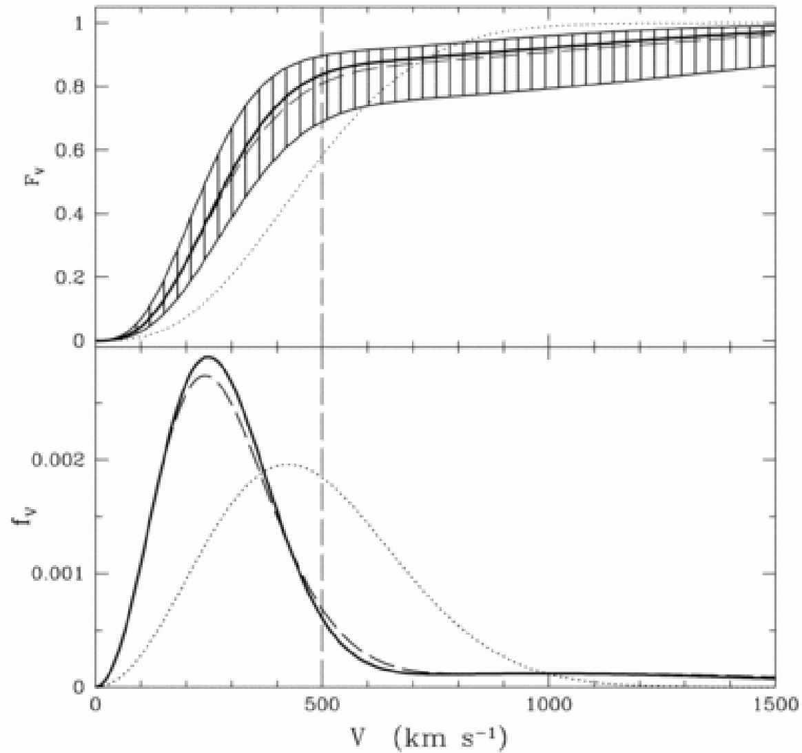
Fig. 7. from Neutron Star Population Dynamics. II. Threedimensional Space Velocities of Young Pulsars Cordes & Chernoff 1998 ApJ 505 315 doi:10.1086/306138 https://dx.doi.org/10.1086/306138 © 1998. The American Astronomical Society. All rights reserved. Printed in U.S.A.
