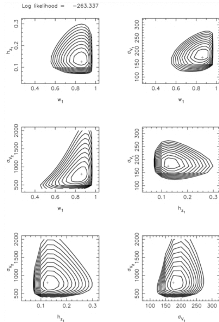
Fig. 5. from Neutron Star Population Dynamics. II. Threedimensional Space Velocities of Young Pulsars Cordes & Chernoff 1998 ApJ 505 315 doi:10.1086/306138 https://dx.doi.org/10.1086/306138 © 1998. The American Astronomical Society. All rights reserved. Printed in U.S.A.
