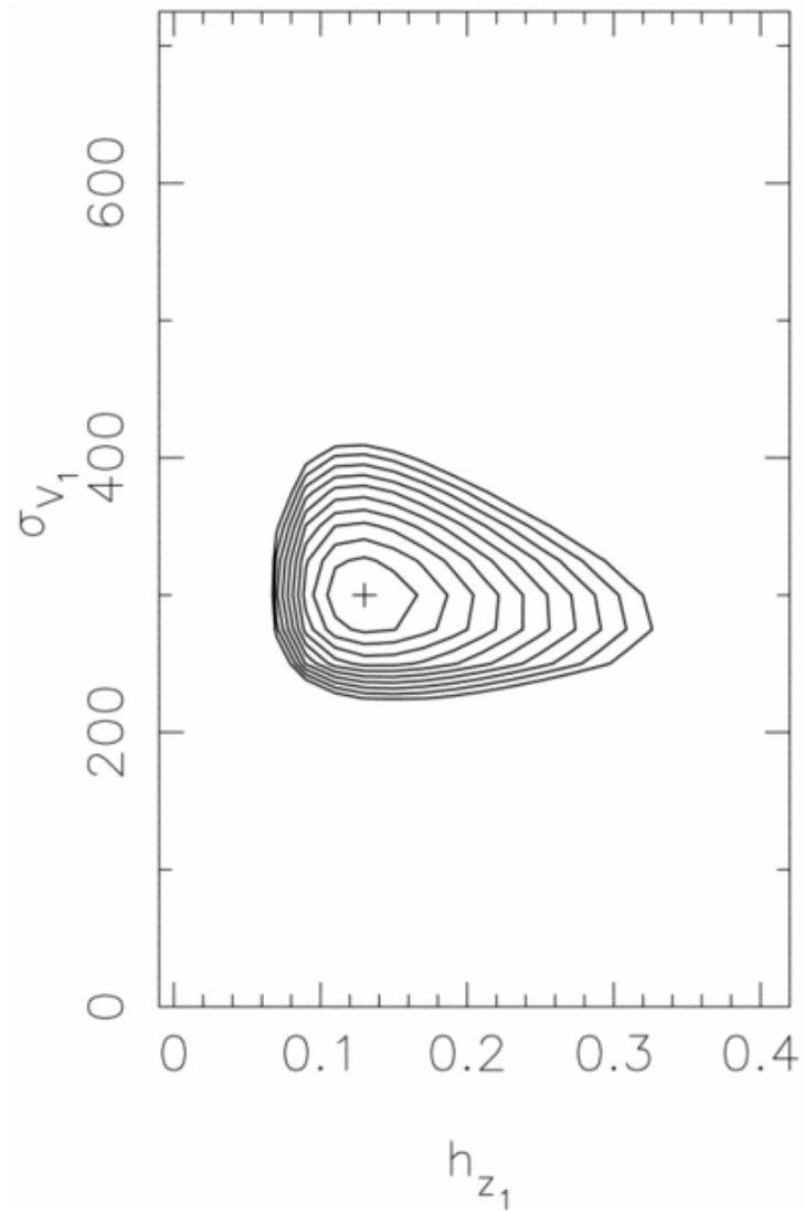
Fig. 4. from Neutron Star Population Dynamics. II. Threedimensional Space Velocities of Young Pulsars Cordes & Chernoff 1998 ApJ 505 315 doi:10.1086/306138 https://dx.doi.org/10.1086/306138 © 1998. The American Astronomical Society. All rights reserved. Printed in U.S.A.
