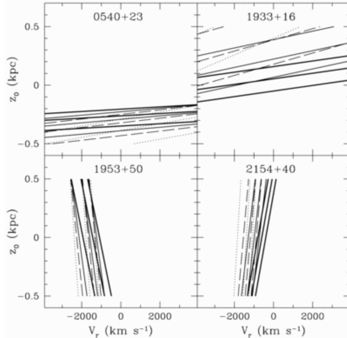
Fig. 3. from Neutron Star Population Dynamics. II. Threedimensional Space Velocities of Young Pulsars Cordes & Chernoff 1998 ApJ 505 315 doi:10.1086/306138 https://dx.doi.org/10.1086/306138 © 1998. The American Astronomical Society. All rights reserved. Printed in U.S.A.
