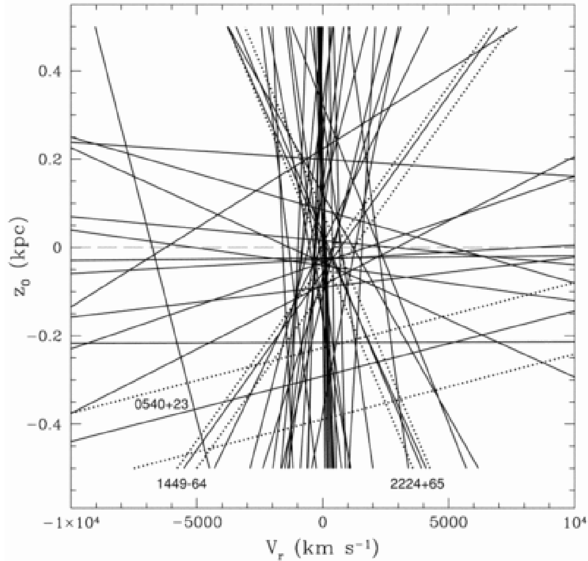
Fig. 2. from Neutron Star Population Dynamics. II. Threedimensional Space Velocities of Young Pulsars Cordes & Chernoff 1998 ApJ 505 315 doi:10.1086/306138 https://dx.doi.org/10.1086/306138 © 1998. The American Astronomical Society. All rights reserved. Printed in U.S.A.
