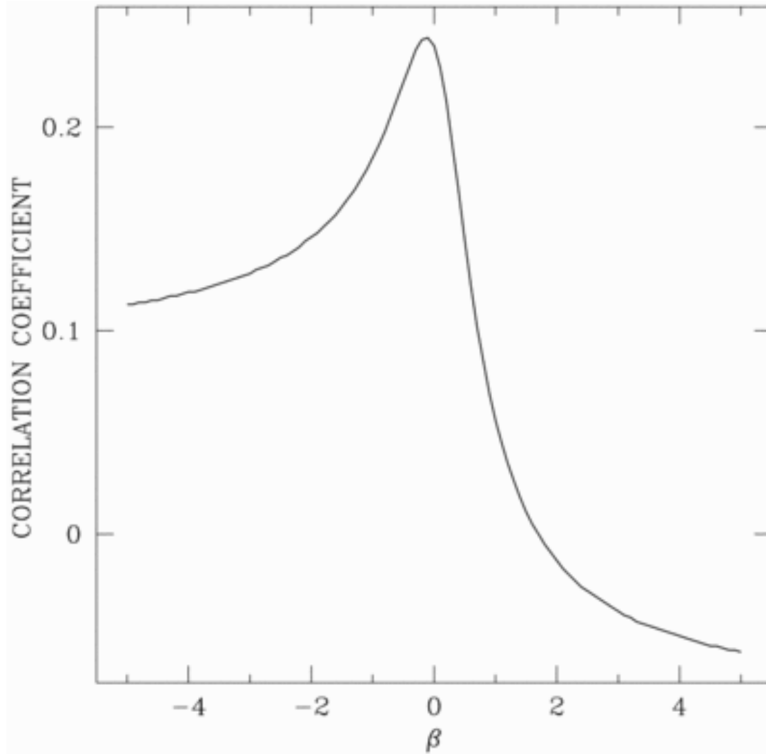
Fig. 13. from Neutron Star Population Dynamics. II. Threedimensional Space Velocities of Young Pulsars Cordes & Chernoff 1998 ApJ 505 315 doi:10.1086/306138 https://dx.doi.org/10.1086/306138 © 1998. The American Astronomical Society. All rights reserved. Printed in U.S.A.
