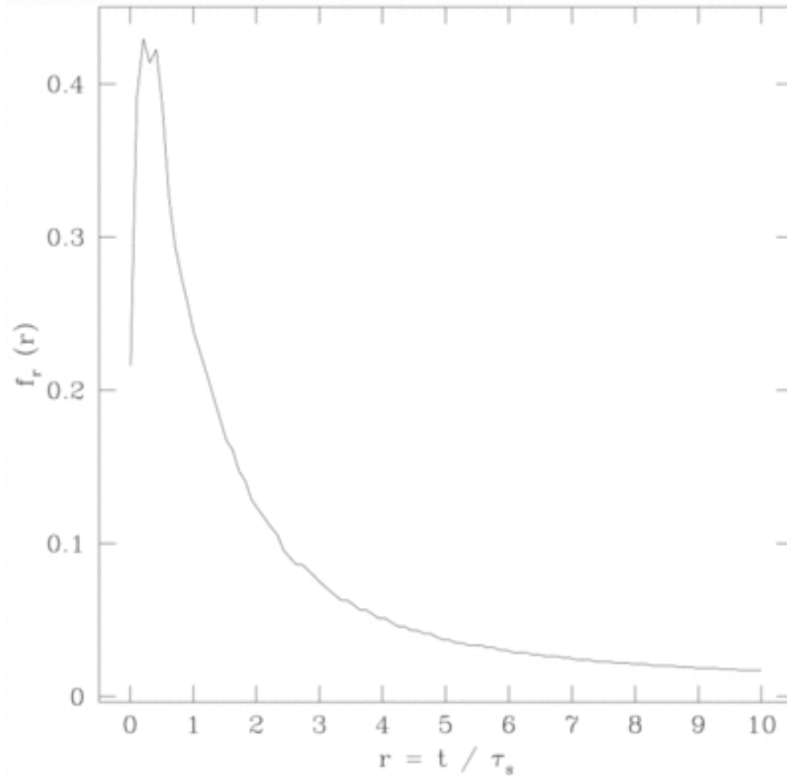
Fig. 12. from Neutron Star Population Dynamics. II. Threedimensional Space Velocities of Young Pulsars Cordes & Chernoff 1998 ApJ 505 315 doi:10.1086/306138 https://dx.doi.org/10.1086/306138 © 1998. The American Astronomical Society. All rights reserved. Printed in U.S.A.
