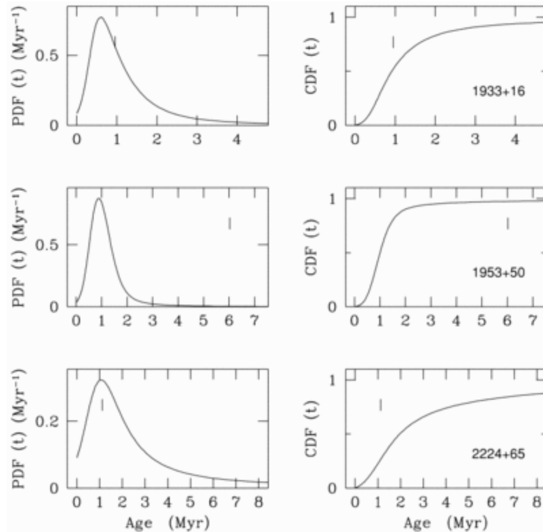
Fig. 10. from Neutron Star Population Dynamics. II. Threedimensional Space Velocities of Young Pulsars Cordes & Chernoff 1998 ApJ 505 315 doi:10.1086/306138 https://dx.doi.org/10.1086/306138 © 1998. The American Astronomical Society. All rights reserved. Printed in U.S.A.
