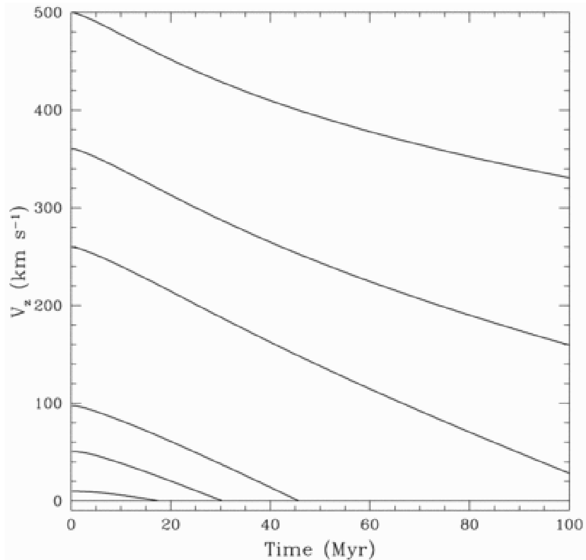
Fig. 1. from Neutron Star Population Dynamics. II. Threedimensional Space Velocities of Young Pulsars Cordes & Chernoff 1998 ApJ 505 315 doi:10.1086/306138 https://dx.doi.org/10.1086/306138 © 1998. The American Astronomical Society. All rights reserved. Printed in U.S.A.
