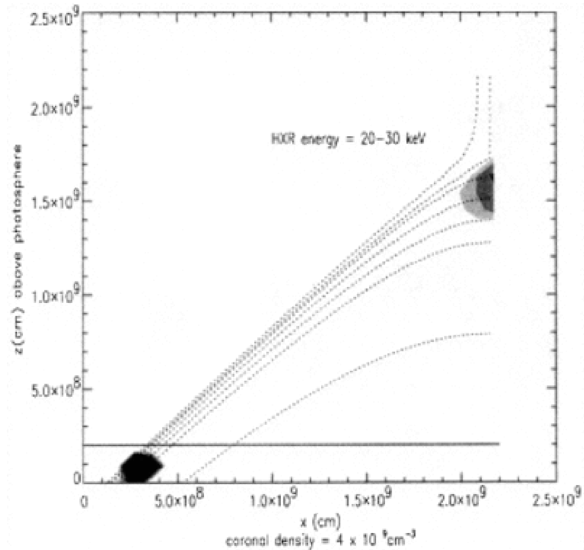
Fig. 8. from A Model for Hard XRay Emission from the Top of Flaring Loops Fletcher & Martens 1998 ApJ 505 418 doi:10.1086/306137 https://dx.doi.org/10.1086/306137 © 1998. The American Astronomical Society. All rights reserved. Printed in U.S.A.
