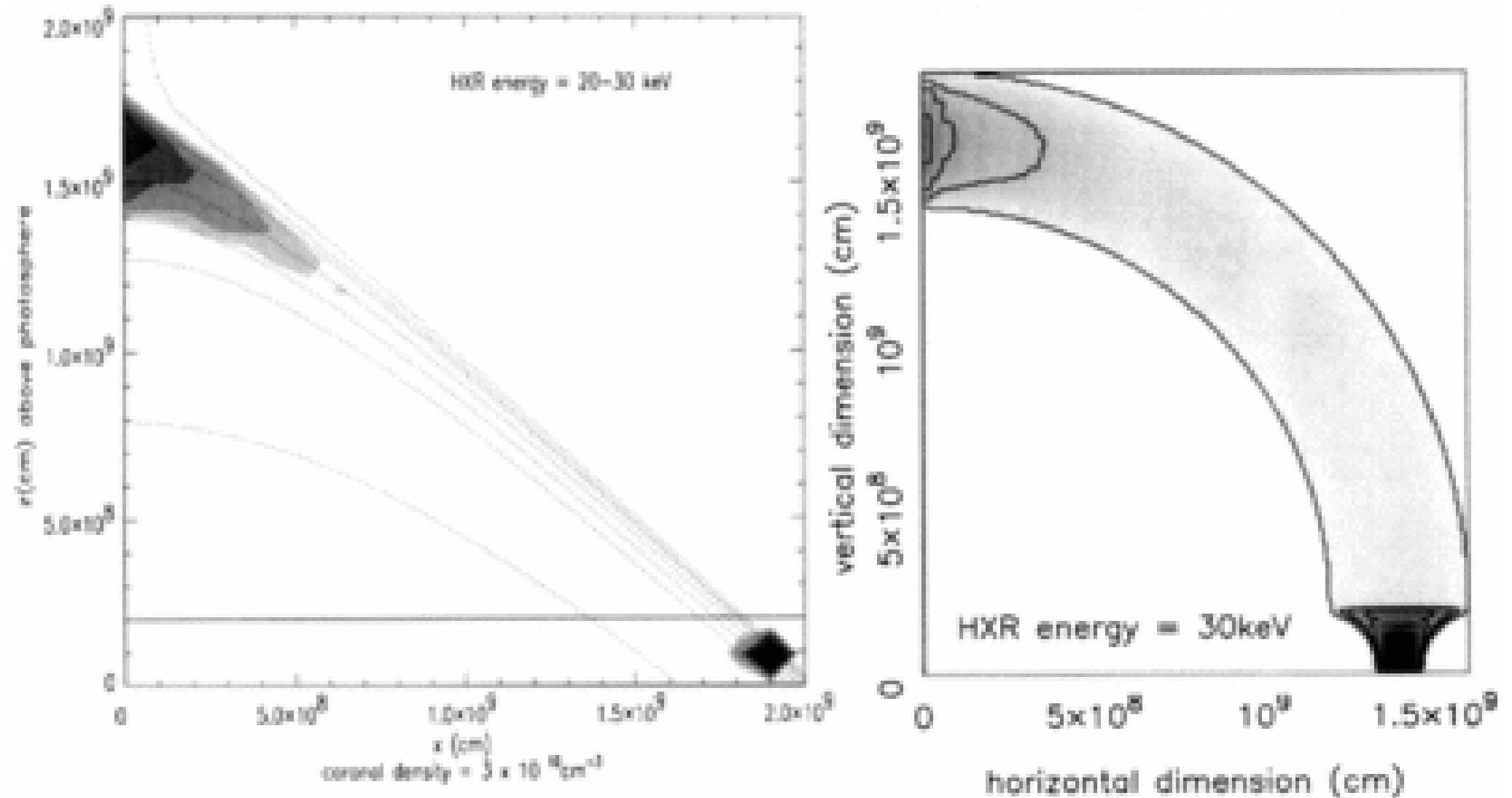
Fig. 5. from A Model for Hard XRay Emission from the Top of Flaring Loops Fletcher & Martens 1998 ApJ 505 418 doi:10.1086/306137 https://dx.doi.org/10.1086/306137 © 1998. The American Astronomical Society. All rights reserved. Printed in U.S.A.
