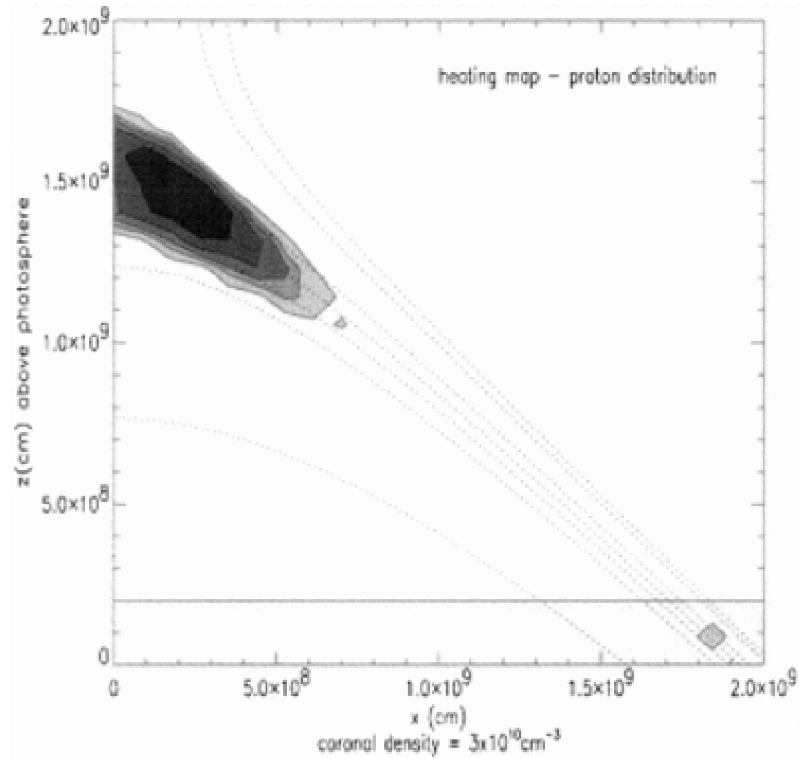
Fig. 10. from A Model for Hard XRay Emission from the Top of Flaring Loops Fletcher & Martens 1998 ApJ 505 418 doi:10.1086/306137 https://dx.doi.org/10.1086/306137 © 1998. The American Astronomical Society. All rights reserved. Printed in U.S.A.
