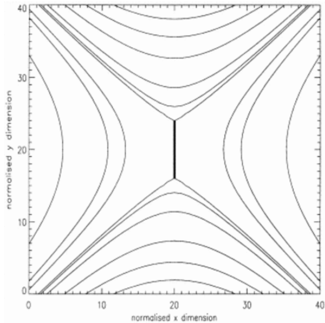
Fig. 1. from A Model for Hard XRay Emission from the Top of Flaring Loops Fletcher & Martens 1998 ApJ 505 418 doi:10.1086/306137 https://dx.doi.org/10.1086/306137 © 1998. The American Astronomical Society. All rights reserved. Printed in U.S.A.
