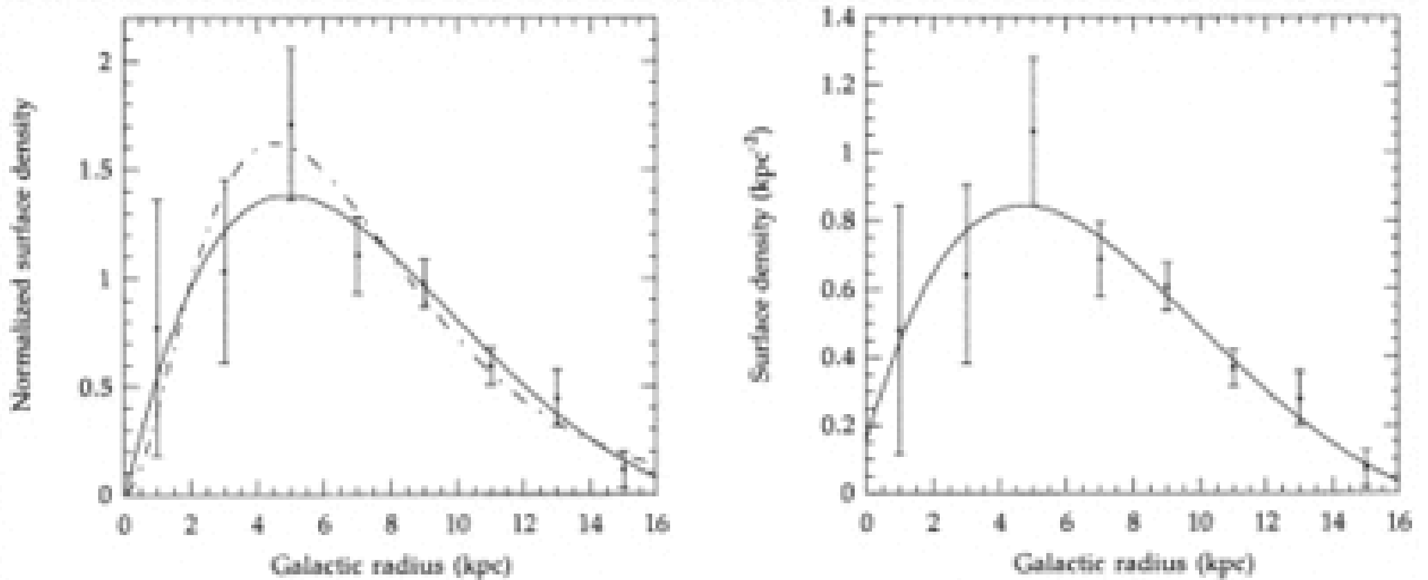
Fig. 7. from A New D Relation and Its Application to the Galactic Supernova Remnant Distribution Case & Bhattacharya 1998 ApJ 504 761 doi:10.1086/306089 https://dx.doi.org/10.1086/306089 © 1998. The American Astronomical Society. All rights reserved. Printed in U.S.A.
