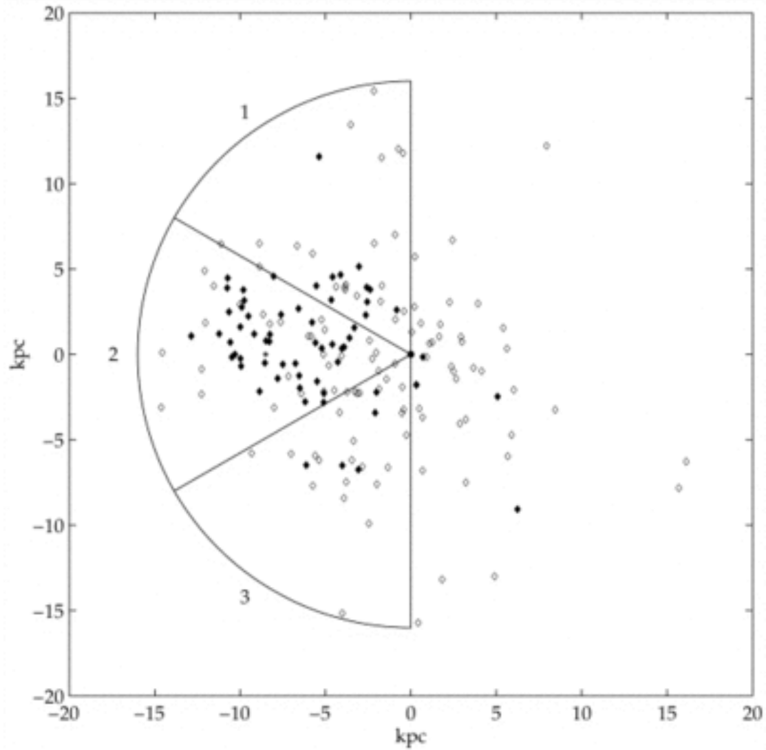
Fig. 6. from A New D Relation and Its Application to the Galactic Supernova Remnant Distribution Case & Bhattacharya 1998 ApJ 504 761 doi:10.1086/306089 https://dx.doi.org/10.1086/306089 © 1998. The American Astronomical Society. All rights reserved. Printed in U.S.A.
