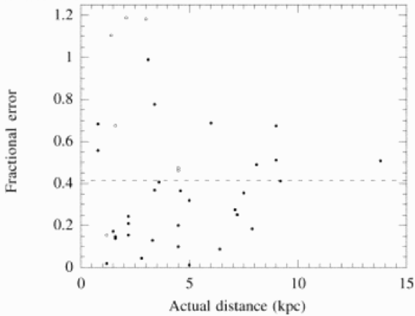
Fig. 3. from A New D Relation and Its Application to the Galactic Supernova Remnant Distribution Case & Bhattacharya 1998 ApJ 504 761 doi:10.1086/306089 https://dx.doi.org/10.1086/306089 © 1998. The American Astronomical Society. All rights reserved. Printed in U.S.A.
