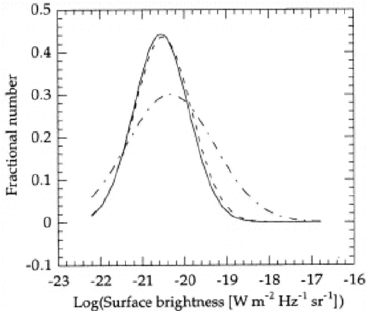
Fig. 2. from A New D Relation and Its Application to the Galactic Supernova Remnant Distribution Case & Bhattacharya 1998 ApJ 504 761 doi:10.1086/306089 https://dx.doi.org/10.1086/306089 © 1998. The American Astronomical Society. All rights reserved. Printed in U.S.A.
