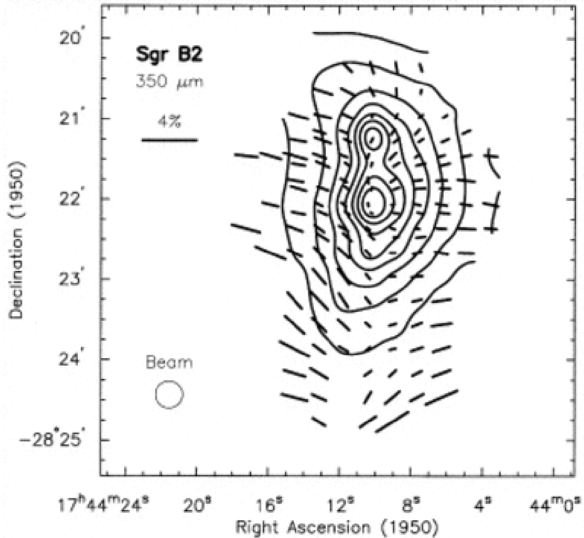
Fig. 7. from Submillimeter Array Polarimetry with Hertz Dowell et al. 1998 ApJ 504 588 doi:10.1086/306069 https://dx.doi.org/10.1086/306069 © 1998. The American Astronomical Society. All rights reserved. Printed in U.S.A.
