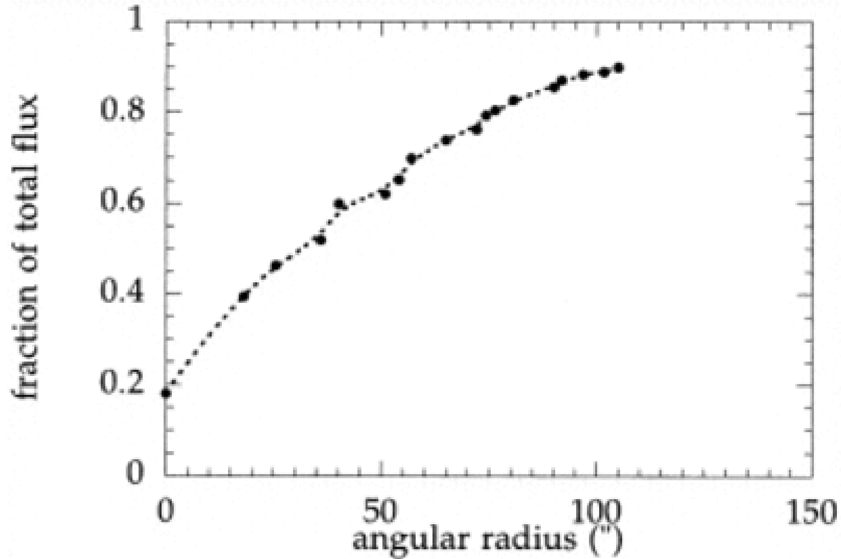
Fig. 4. from Submillimeter Array Polarimetry with Hertz Dowell et al. 1998 ApJ 504 588 doi:10.1086/306069 https://dx.doi.org/10.1086/306069 © 1998. The American Astronomical Society. All rights reserved. Printed in U.S.A.
