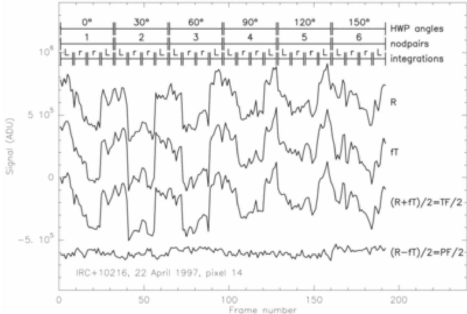
Fig. 2. from Submillimeter Array Polarimetry with Hertz Dowell et al. 1998 ApJ 504 588 doi:10.1086/306069 https://dx.doi.org/10.1086/306069 © 1998. The American Astronomical Society. All rights reserved. Printed in U.S.A.
