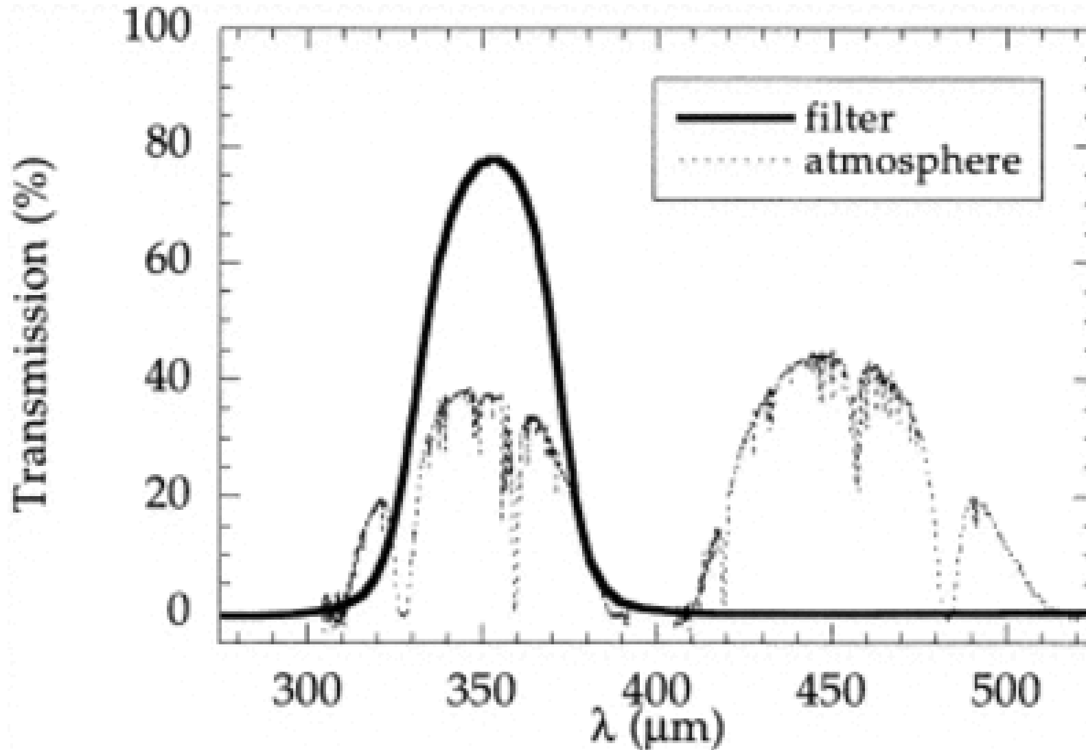
Fig. 1. from Submillimeter Array Polarimetry with Hertz Dowell et al. 1998 ApJ 504 588 doi:10.1086/306069 https://dx.doi.org/10.1086/306069 © 1998. The American Astronomical Society. All rights reserved. Printed in U.S.A.
