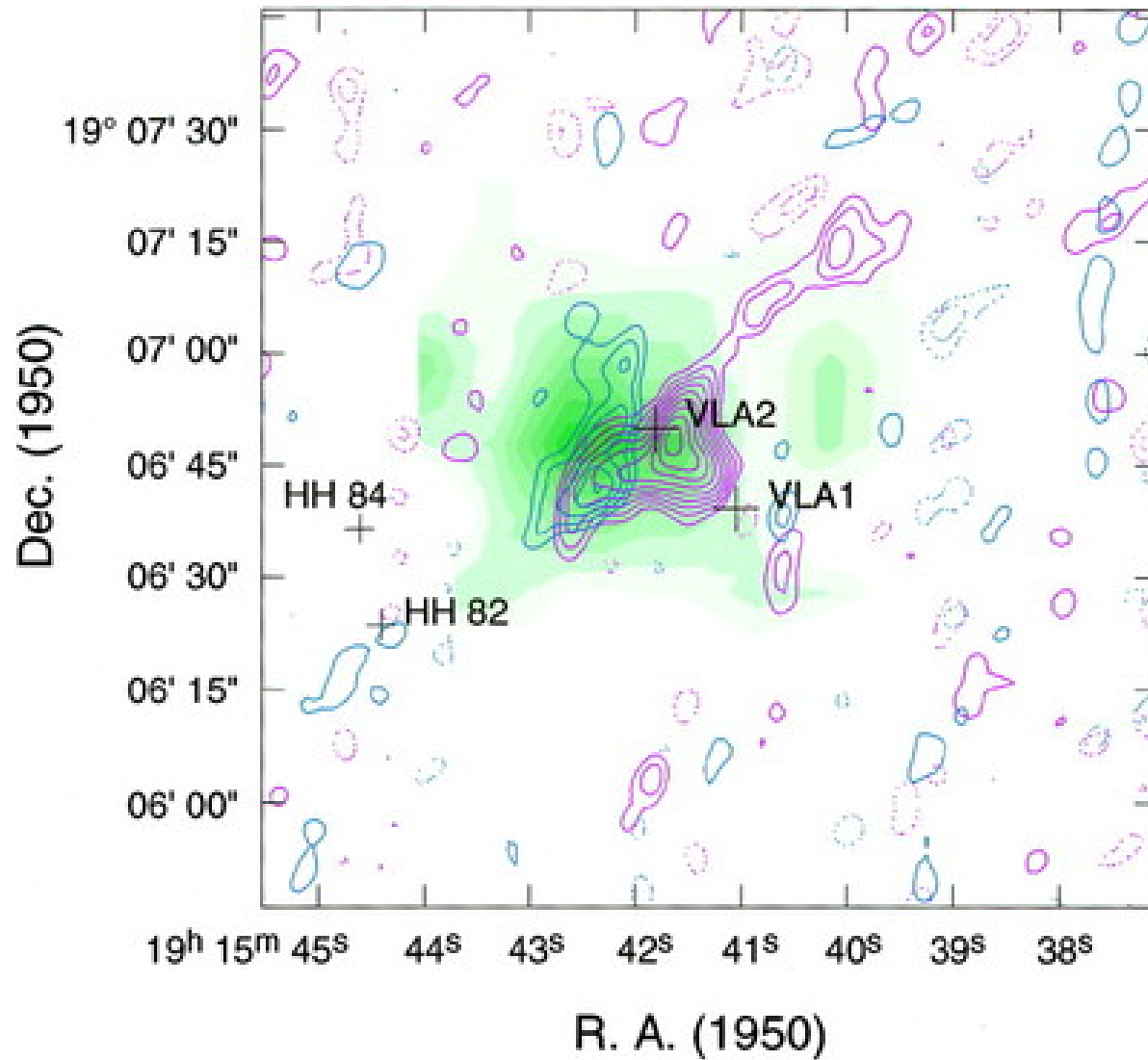
Fig. 4. from The Powering Source and Origin of the Quadrupolar Molecular Outflow in L723 Hirano et al. 1998 ApJ 504 334 doi:10.1086/306068 https://dx.doi.org/10.1086/306068 © 1998. The American Astronomical Society. All rights reserved. Printed in U.S.A.
