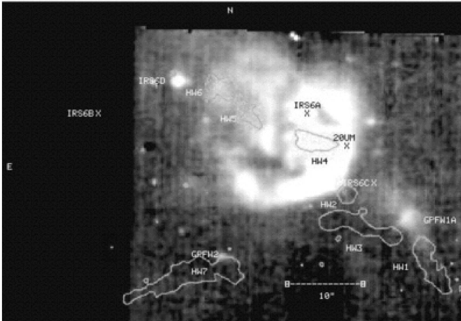
Fig. 6. from Cepheus A East: Unraveling the Mysteries Goetz et al. 1998 ApJ 504 359 doi:10.1086/306058 https://dx.doi.org/10.1086/306058 © 1998. The American Astronomical Society. All rights reserved. Printed in U.S.A.
