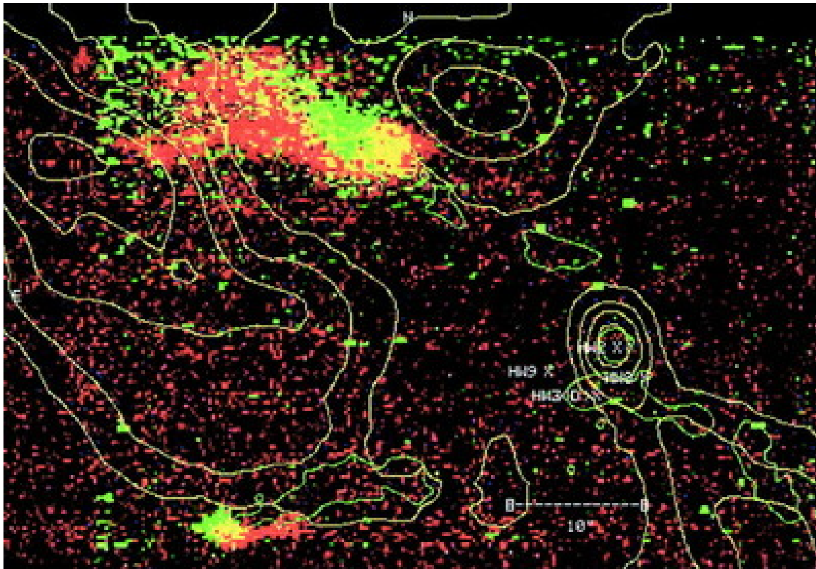
Fig. 4. from Cepheus A East: Unraveling the Mysteries Goetz et al. 1998 ApJ 504 359 doi:10.1086/306058 https://dx.doi.org/10.1086/306058 © 1998. The American Astronomical Society. All rights reserved. Printed in U.S.A.
