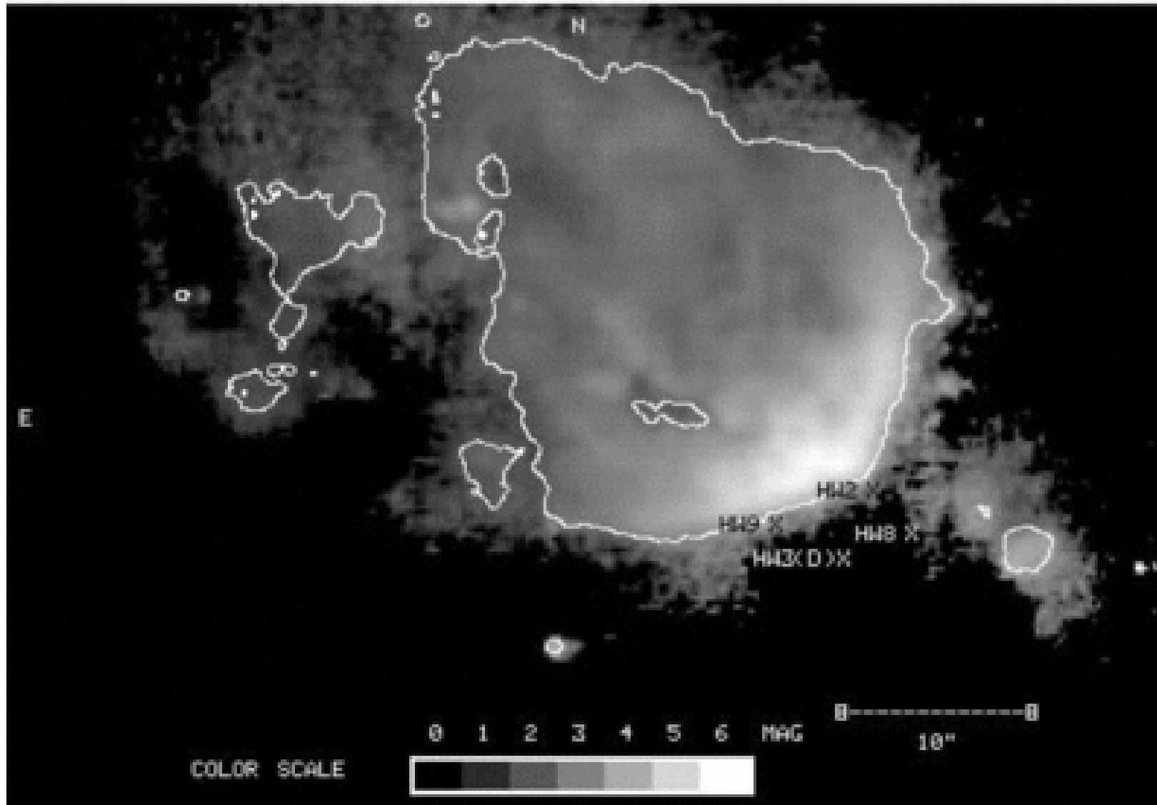
Fig. 3. from Cepheus A East: Unraveling the Mysteries Goetz et al. 1998 ApJ 504 359 doi:10.1086/306058 https://dx.doi.org/10.1086/306058 © 1998. The American Astronomical Society. All rights reserved. Printed in U.S.A.
