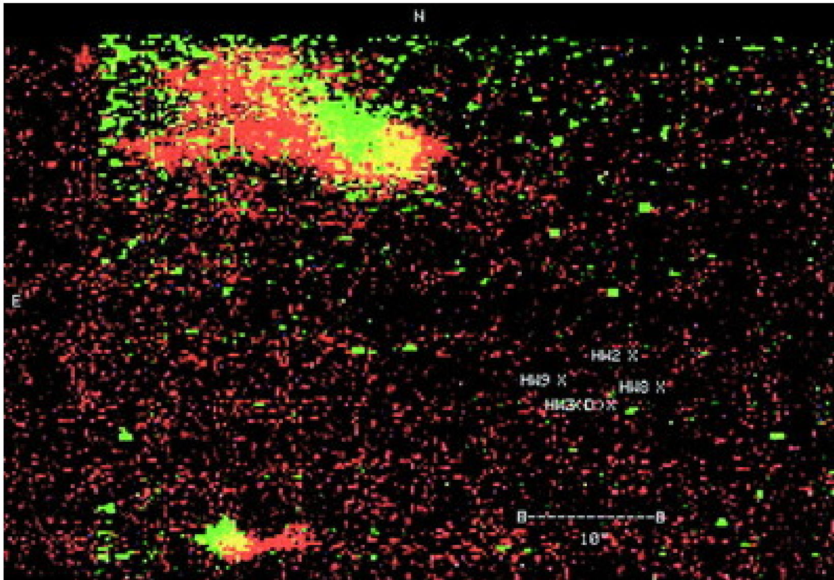
Fig. 2. from Cepheus A East: Unraveling the Mysteries Goetz et al. 1998 ApJ 504 359 doi:10.1086/306058 https://dx.doi.org/10.1086/306058 © 1998. The American Astronomical Society. All rights reserved. Printed in U.S.A.
