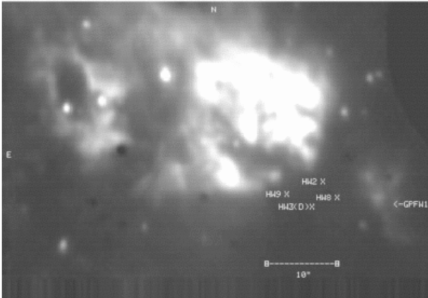
Fig. 1. from Cepheus A East: Unraveling the Mysteries Goetz et al. 1998 ApJ 504 359 doi:10.1086/306058 https://dx.doi.org/10.1086/306058 © 1998. The American Astronomical Society. All rights reserved. Printed in U.S.A.
