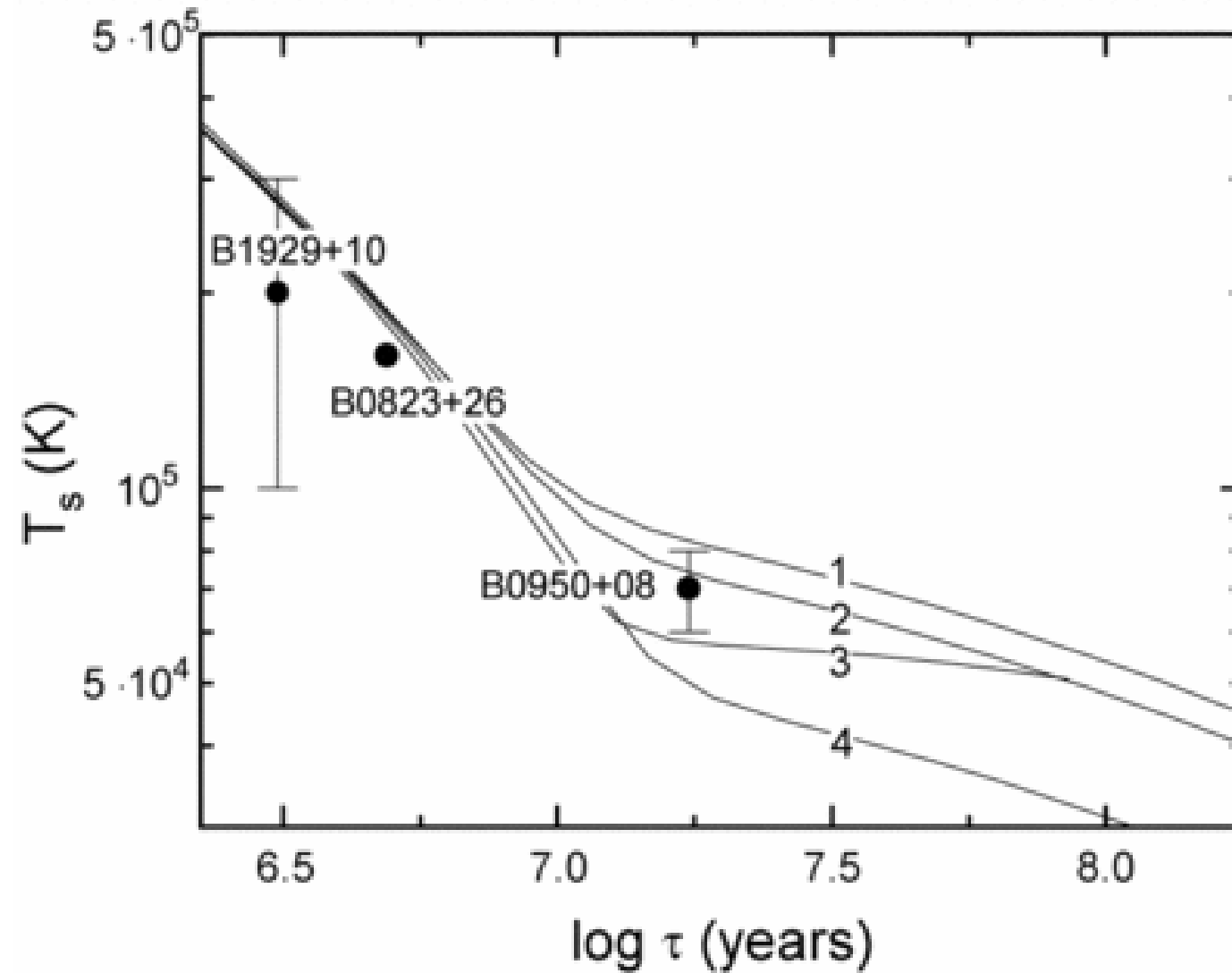
Fig. 5. from Joule Heating and the Thermal Evolution of Old Neutron Stars Miralles, Urpin, & Konenkov 1998 ApJ 503 368 doi:10.1086/305967 https://dx.doi.org/10.1086/305967 © 1998. The American Astronomical Society. All rights reserved. Printed in U.S.A.
