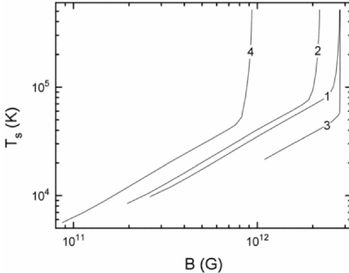
Fig. 4. from Joule Heating and the Thermal Evolution of Old Neutron Stars Miralles, Urpin, & Konenkov 1998 ApJ 503 368 doi:10.1086/305967 https://dx.doi.org/10.1086/305967 © 1998. The American Astronomical Society. All rights reserved. Printed in U.S.A.
