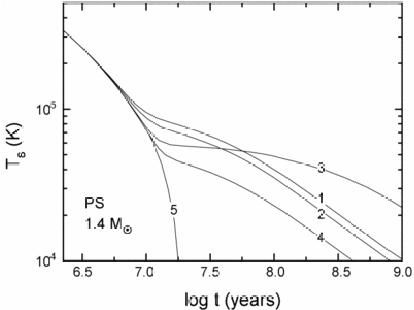
Fig. 3. from Joule Heating and the Thermal Evolution of Old Neutron Stars Miralles, Urpin, & Konenkov 1998 ApJ 503 368 doi:10.1086/305967 https://dx.doi.org/10.1086/305967 © 1998. The American Astronomical Society. All rights reserved. Printed in U.S.A.
