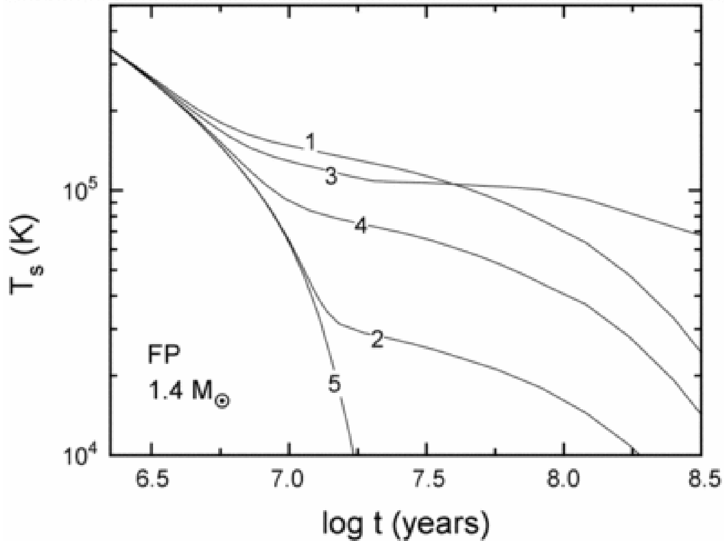
Fig. 2. from Joule Heating and the Thermal Evolution of Old Neutron Stars Miralles, Urpin, & Konenkov 1998 ApJ 503 368 doi:10.1086/305967 https://dx.doi.org/10.1086/305967 © 1998. The American Astronomical Society. All rights reserved. Printed in U.S.A.
