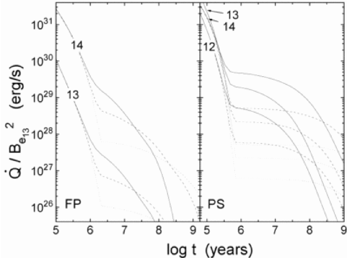
Fig. 1. from Joule Heating and the Thermal Evolution of Old Neutron Stars Miralles, Urpin, & Konenkov 1998 ApJ 503 368 doi:10.1086/305967 https://dx.doi.org/10.1086/305967 © 1998. The American Astronomical Society. All rights reserved. Printed in U.S.A.
