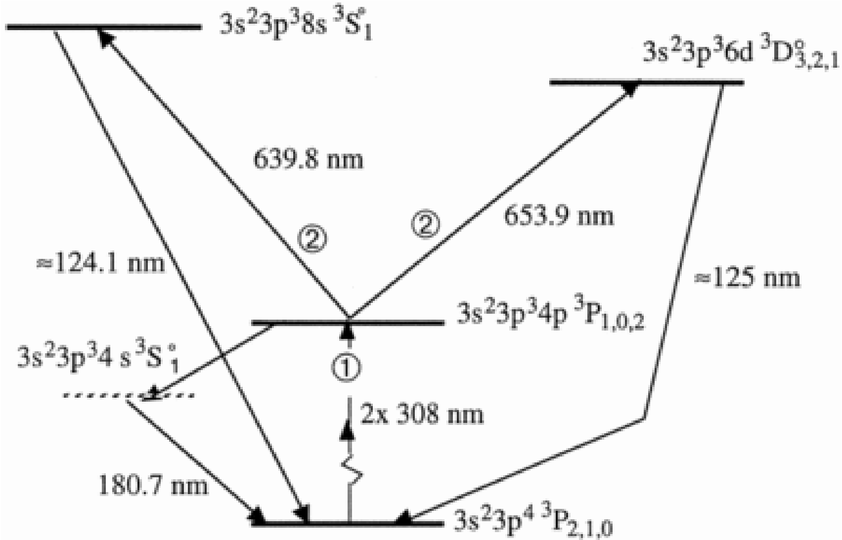
Fig. 1. from Lifetimes and Oscillator Strengths for Ultraviolet Transitions in Neutral Sulfur Biémont et al. 1998 ApJ 502 1010 doi:10.1086/305943 https://dx.doi.org/10.1086/305943 © 1998. The American Astronomical Society. All rights reserved. Printed in U.S.A.
