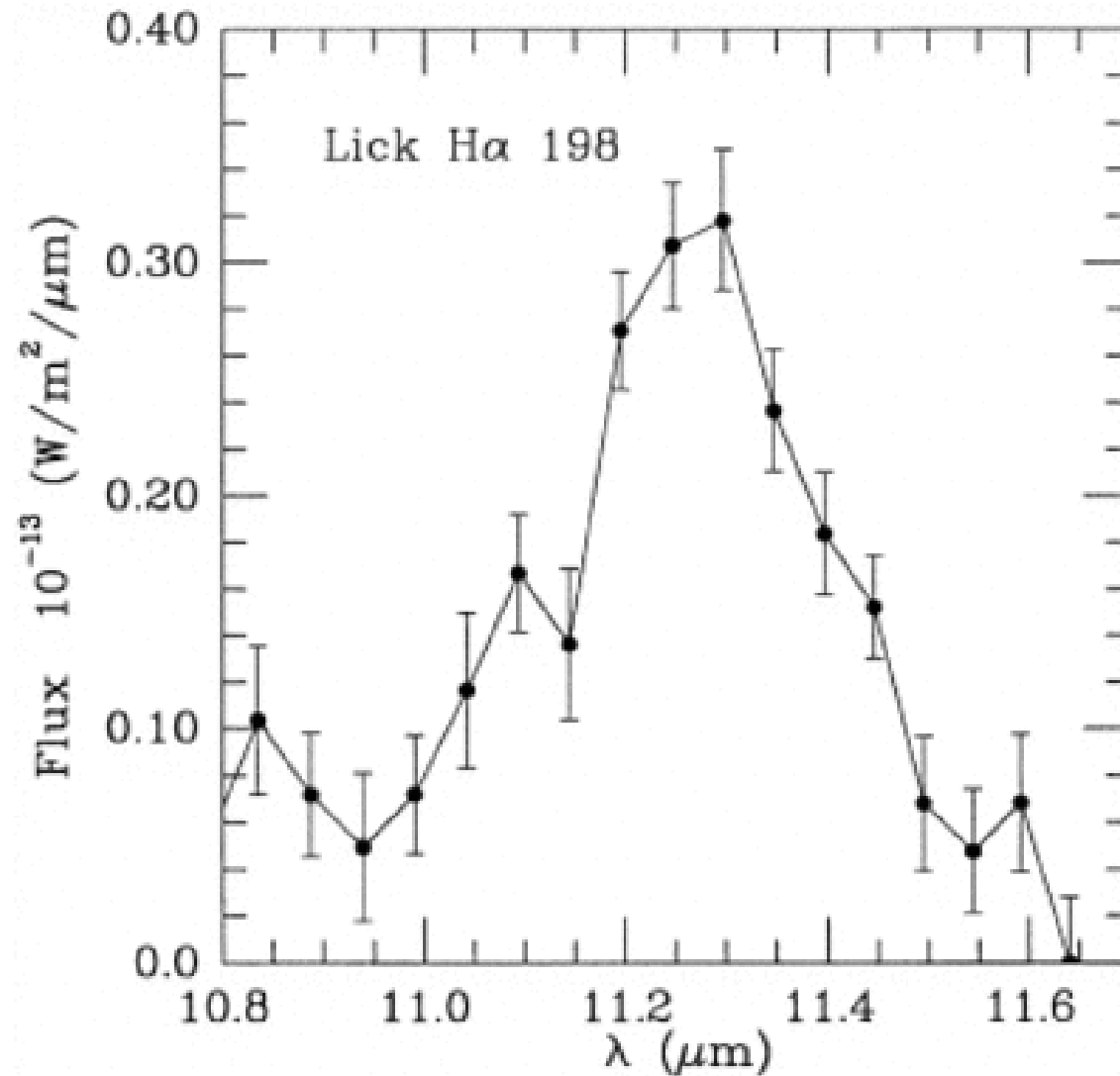
Fig. 7. from 8–13 Micron Spectroscopy of Young Stars Hanner, Brooke, & Tokunaga 1998 ApJ 502 871 doi:10.1086/305939 https://dx.doi.org/10.1086/305939 © 1998. The American Astronomical Society. All rights reserved. Printed in U.S.A.
