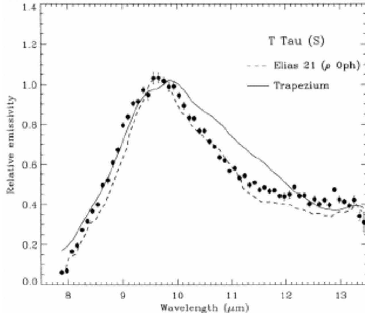
Fig. 5. from 8–13 Micron Spectroscopy of Young Stars Hanner, Brooke, & Tokunaga 1998 ApJ 502 871 doi:10.1086/305939 https://dx.doi.org/10.1086/305939 © 1998. The American Astronomical Society. All rights reserved. Printed in U.S.A.
