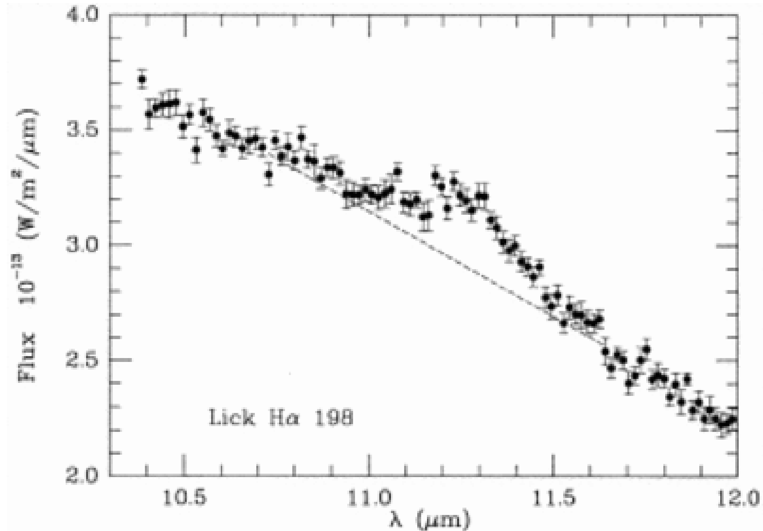
Fig. 6. from 8–13 Micron Spectroscopy of Young Stars Hanner, Brooke, & Tokunaga 1998 ApJ 502 871 doi:10.1086/305939 https://dx.doi.org/10.1086/305939 © 1998. The American Astronomical Society. All rights reserved. Printed in U.S.A.
