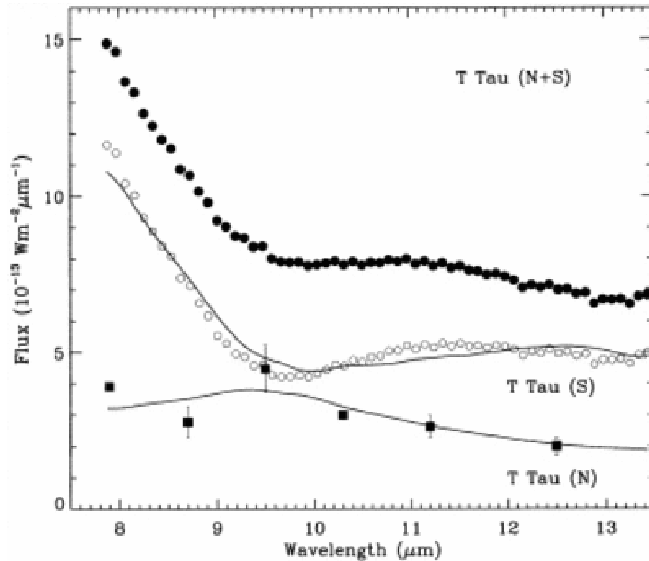
Fig. 4. from 8–13 Micron Spectroscopy of Young Stars Hanner, Brooke, & Tokunaga 1998 ApJ 502 871 doi:10.1086/305939 https://dx.doi.org/10.1086/305939 © 1998. The American Astronomical Society. All rights reserved. Printed in U.S.A.
