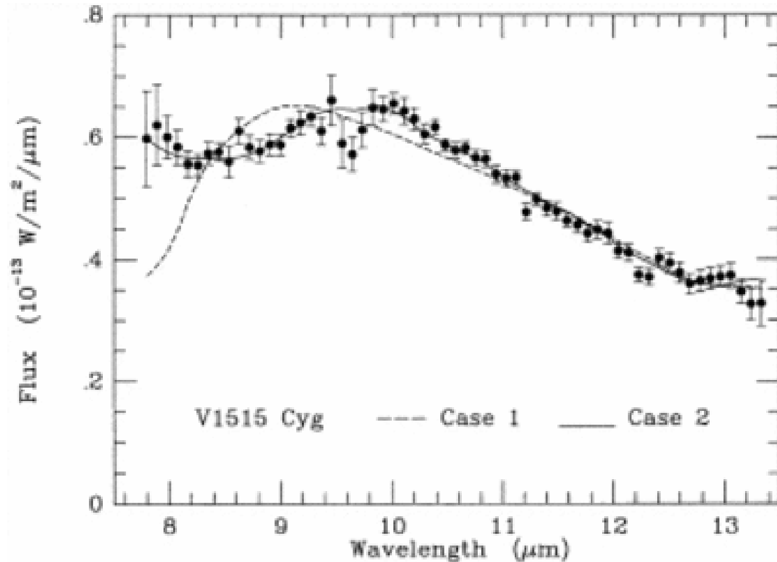
Fig. 3. from 8–13 Micron Spectroscopy of Young Stars Hanner, Brooke, & Tokunaga 1998 ApJ 502 871 doi:10.1086/305939 https://dx.doi.org/10.1086/305939 © 1998. The American Astronomical Society. All rights reserved. Printed in U.S.A.
