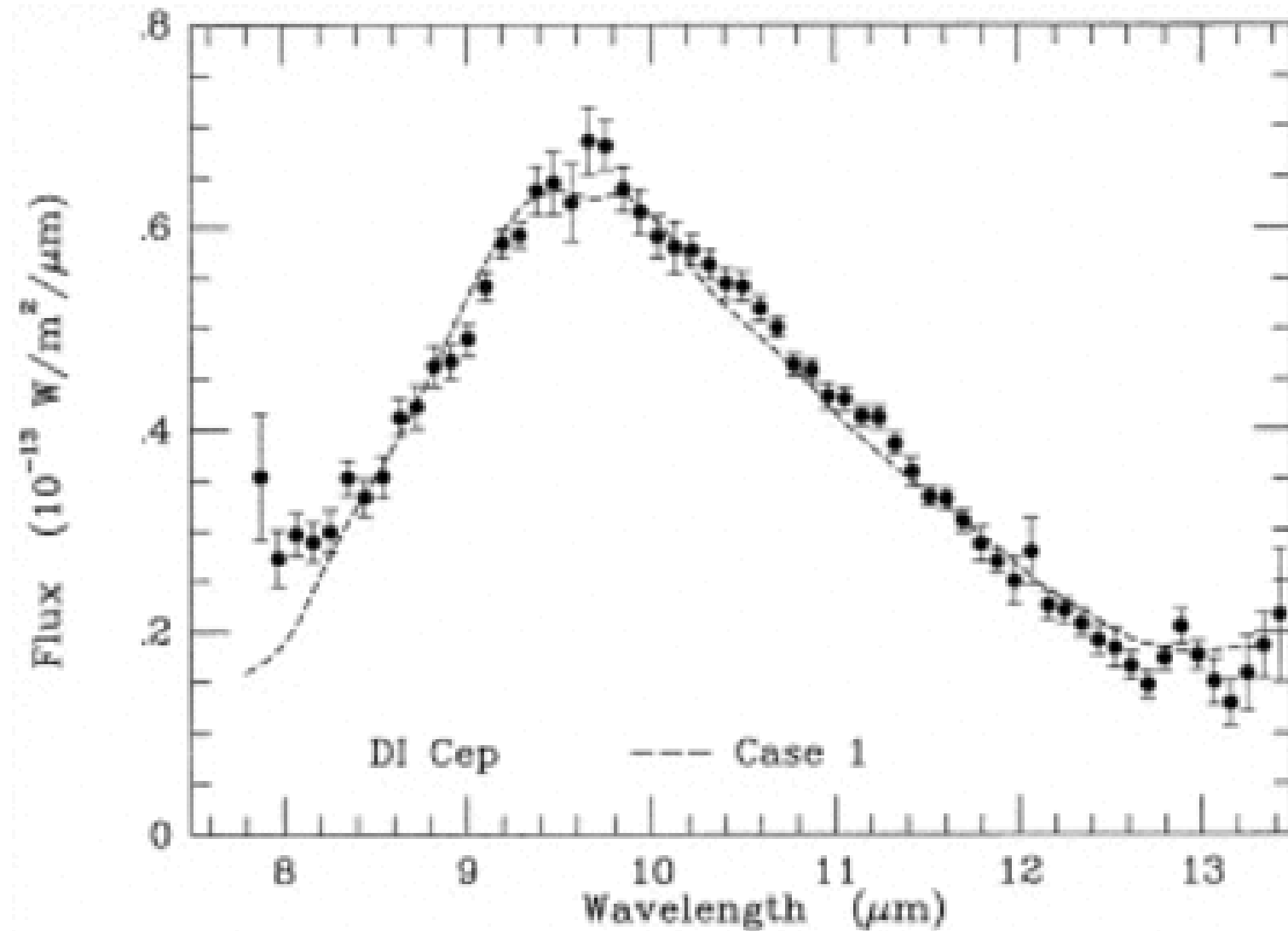
Fig. 2. from 8–13 Micron Spectroscopy of Young Stars Hanner, Brooke, & Tokunaga 1998 ApJ 502 871 doi:10.1086/305939 https://dx.doi.org/10.1086/305939 © 1998. The American Astronomical Society. All rights reserved. Printed in U.S.A.
