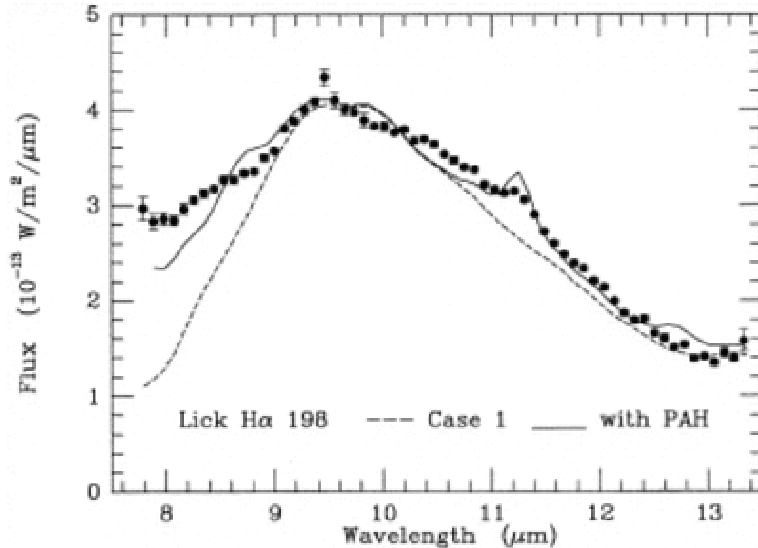
Fig. 1. from 8–13 Micron Spectroscopy of Young Stars Hanner, Brooke, & Tokunaga 1998 ApJ 502 871 doi:10.1086/305939 https://dx.doi.org/10.1086/305939 © 1998. The American Astronomical Society. All rights reserved. Printed in U.S.A.
