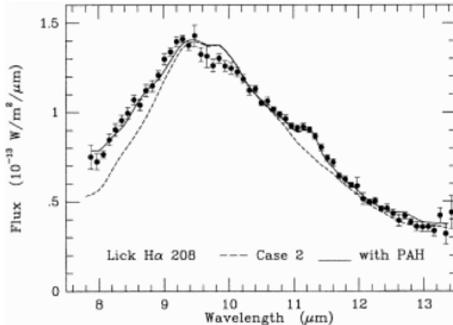
Fig. 1. from 8–13 Micron Spectroscopy of Young Stars Hanner, Brooke, & Tokunaga 1998 ApJ 502 871 doi:10.1086/305939 https://dx.doi.org/10.1086/305939 © 1998. The American Astronomical Society. All rights reserved. Printed in U.S.A.
