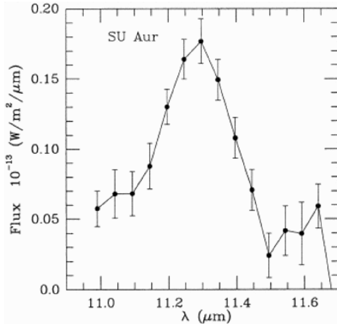
Fig. 8. from 8–13 Micron Spectroscopy of Young Stars Hanner, Brooke, & Tokunaga 1998 ApJ 502 871 doi:10.1086/305939 https://dx.doi.org/10.1086/305939 © 1998. The American Astronomical Society. All rights reserved. Printed in U.S.A.
