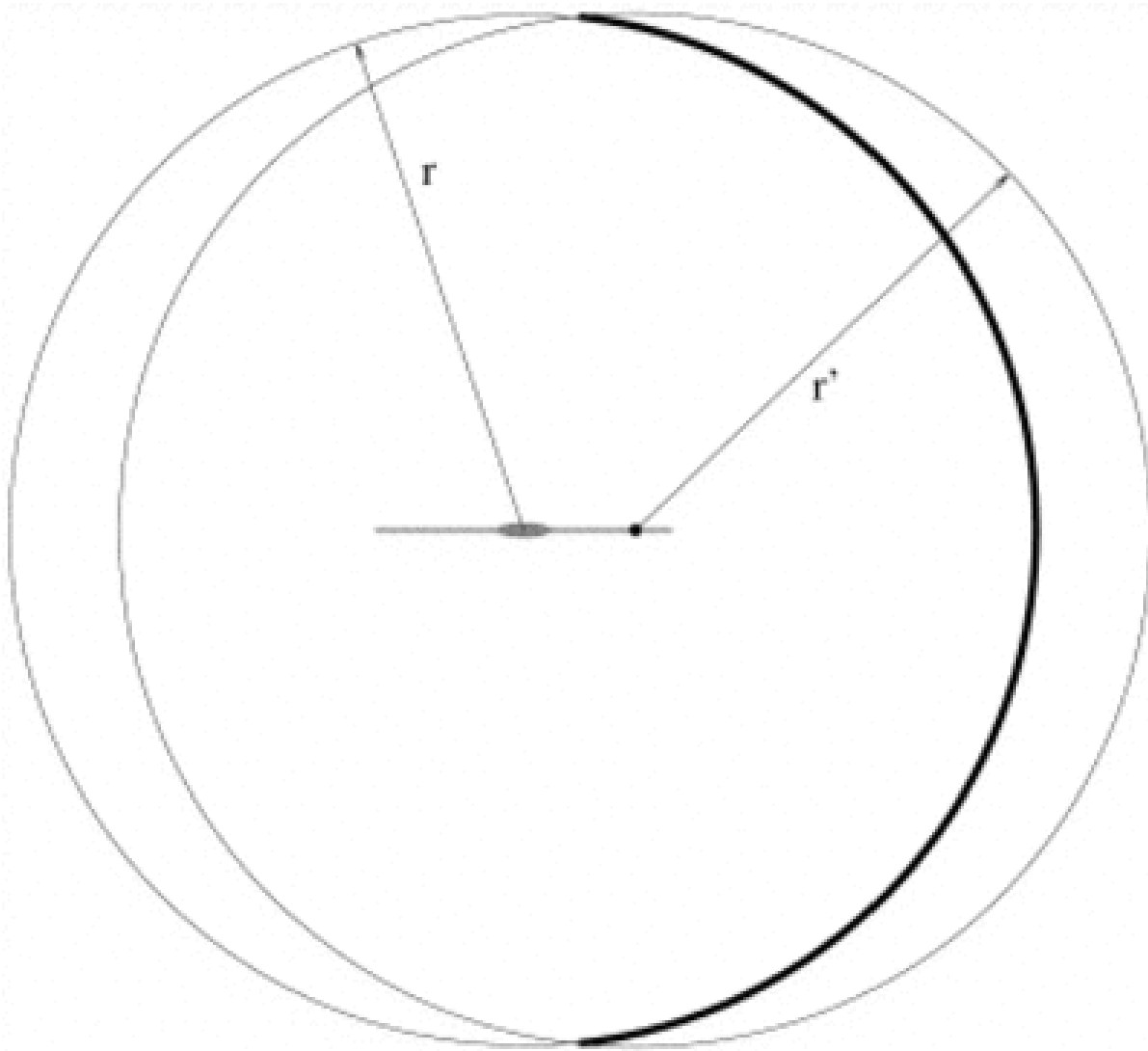
Fig. 7. from Inferring the Spatial and Energy Distribution of GammaRay Burst Sources. III. Anisotropic Models Loredo & Wasserman 1998 ApJ 502 108 doi:10.1086/305871 https://dx.doi.org/10.1086/305871 © 1998. The American Astronomical Society. All rights reserved. Printed in U.S.A.
