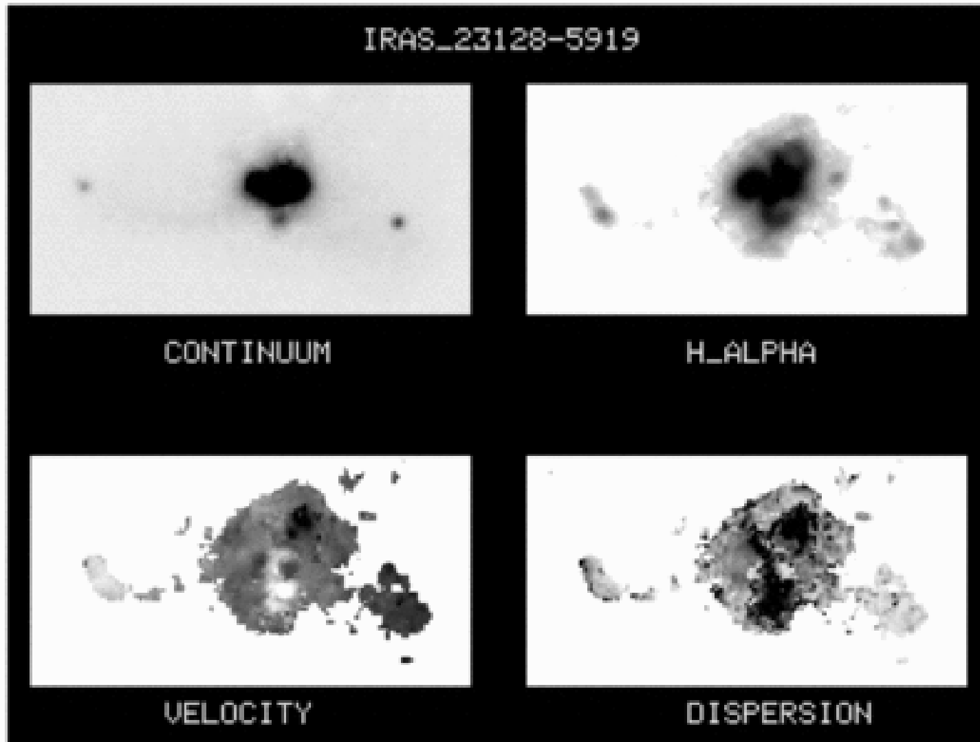
Fig. 9. from H Velocity Mapping of Ultraluminous Infrared Galaxies Mihos & Bothun 1998 ApJ 500 619 doi:10.1086/305747 https://dx.doi.org/10.1086/305747 © 1998. The American Astronomical Society. All rights reserved. Printed in U.S.A.
