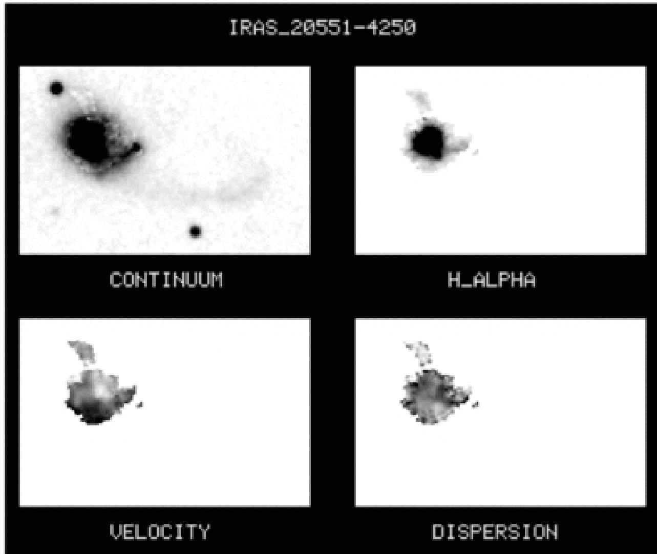
Fig. 7. from H Velocity Mapping of Ultraluminous Infrared Galaxies Mihos & Bothun 1998 ApJ 500 619 doi:10.1086/305747 https://dx.doi.org/10.1086/305747 © 1998. The American Astronomical Society. All rights reserved. Printed in U.S.A.
