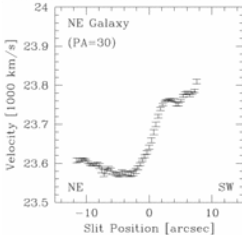
Fig. 3. from H Velocity Mapping of Ultraluminous Infrared Galaxies Mihos & Bothun 1998 ApJ 500 619 doi:10.1086/305747 https://dx.doi.org/10.1086/305747 © 1998. The American Astronomical Society. All rights reserved. Printed in U.S.A.
