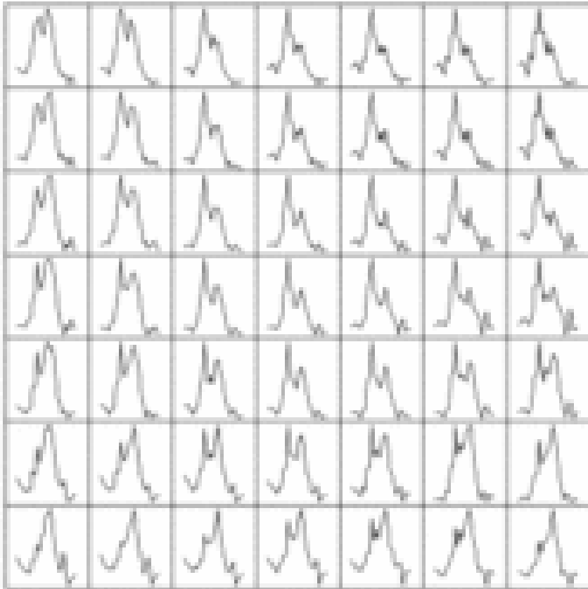
Fig. 11. from H Velocity Mapping of Ultraluminous Infrared Galaxies Mihos & Bothun 1998 ApJ 500 619 doi:10.1086/305747 https://dx.doi.org/10.1086/305747 © 1998. The American Astronomical Society. All rights reserved. Printed in U.S.A.
